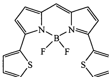
Comparative Compound 1
