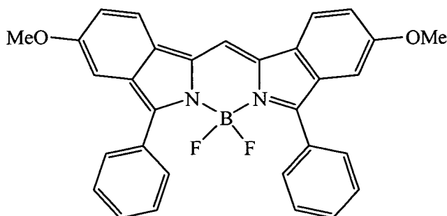
Comparative Compound 2
